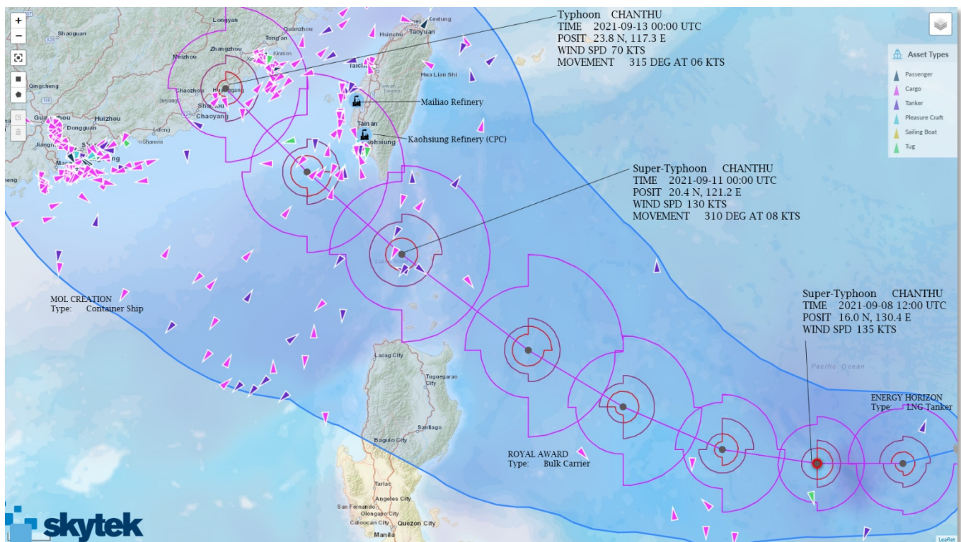
Figure 1 - aggregated exposure in the cone of Super-Typhoon Chanthu, Sep 8th, 2021
